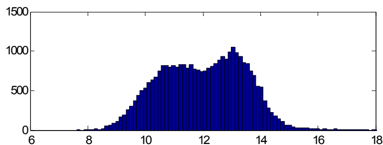
Figure 2. Frame log-energy histograms calculated over the whole seminar signal
